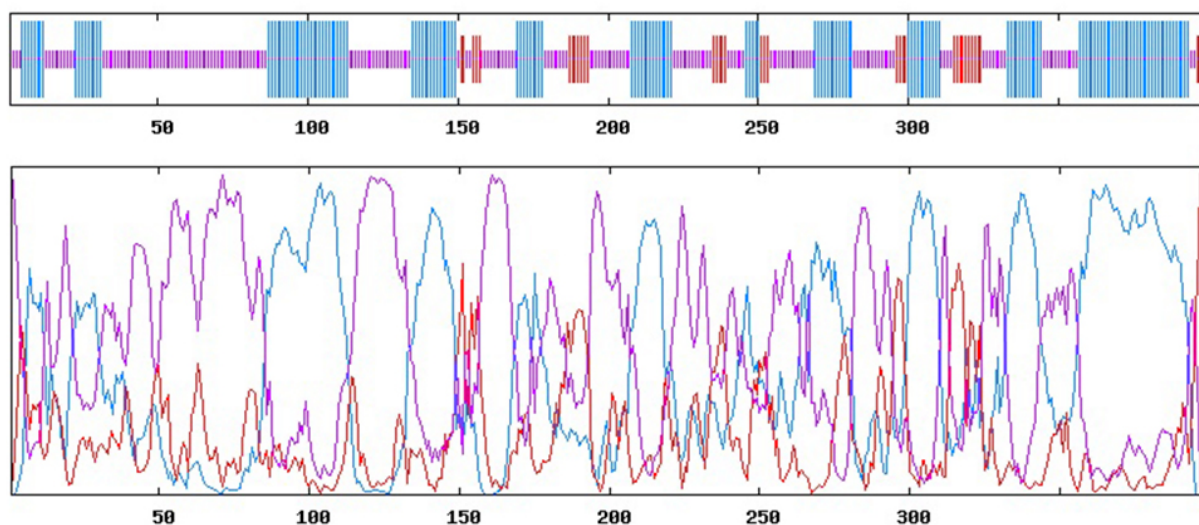
Figure 3. A) Predicted secondary structure by the GOR IV online service [70]; B) Graphical results for secondary structure prediction of ROP13 protein by GOR IV
