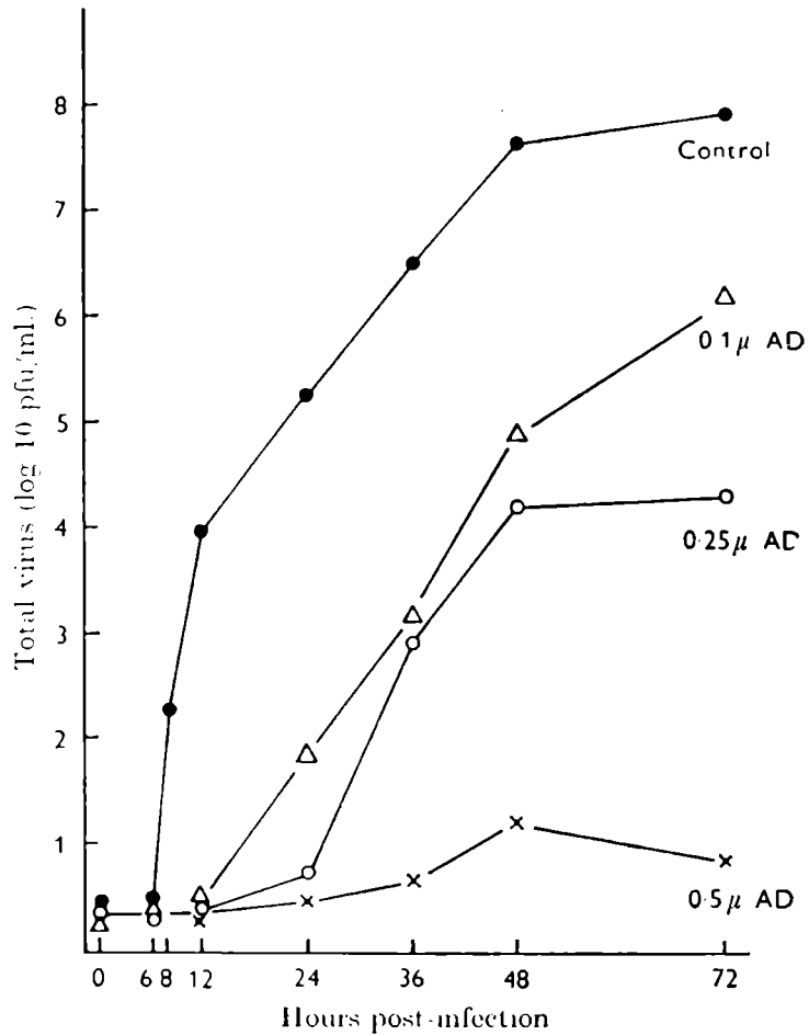
Fig. 1 Growth of African horse sickness virus type 6, strain 114 in MS cells infected at a multiplicity of 2. Cells pretreated with: Δ, actinomyein D 0.1 μg./ml., ○, AD 0.25 μg./ml., ×, AD 0.5 μg./ml., ●, untreated control
