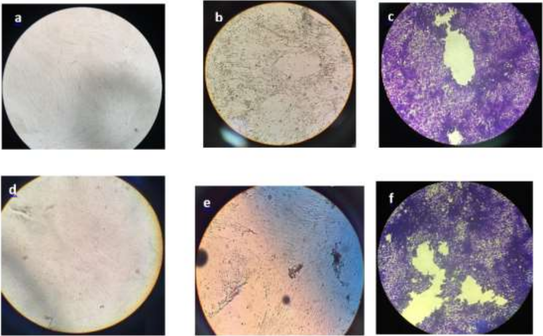
Figure 4: a) An uninfected RHDC cell showing no signs of cytopathic effect. b) RHDC 4 days post-infection. c) RHDC 4 days post-infection stained with crystal violet. d) An uninfected MRC-5 cell showing no signs of cytopathic effect. e) MRC-5 4 days post-infection. f) MRC-5 4 days post-infection stained with crystal violet
