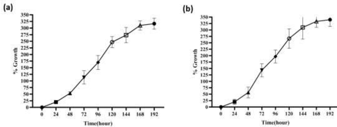
Figure 1: Growth curve of RHDC (a) and MRC-5 (b) cells under static culture conditions. Cell counts in flasks are plotted against incubation time. Cells were cultured in DMEM with 7% FBS in a 25 cm 2 flask.
